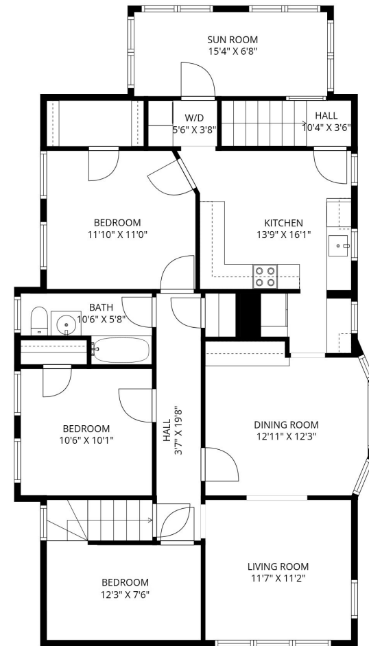
7 PEARL STREET FLOOR 2
